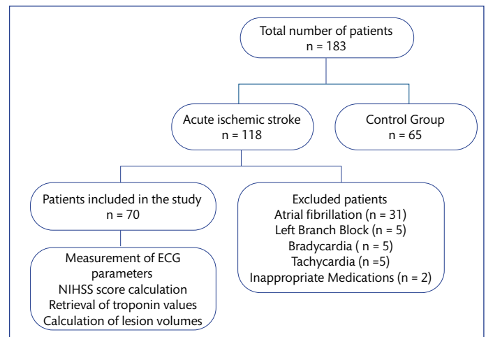
Figure 3. Study flowchart.
